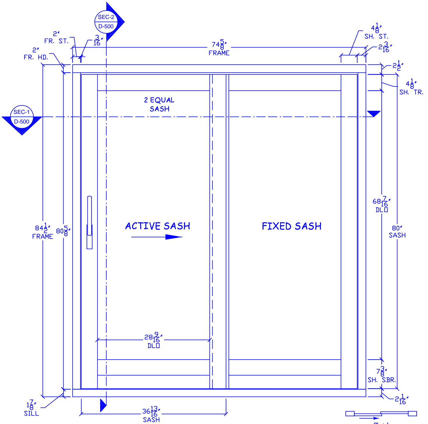
2-PANEL LIFT-SLIDE DOOR (1 Active, 1 Fixed - Stacked Bottom-Rail)
