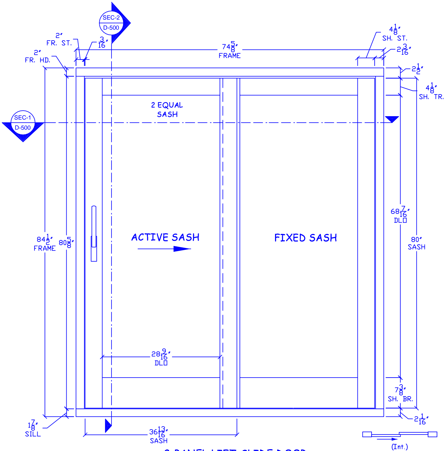
2-PANEL LIFT-SLIDE DOOR (1 Active, 1 Fixed - Solid Bottom-Rail)
